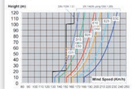
Wind Speed profile depending on the height from the ground
